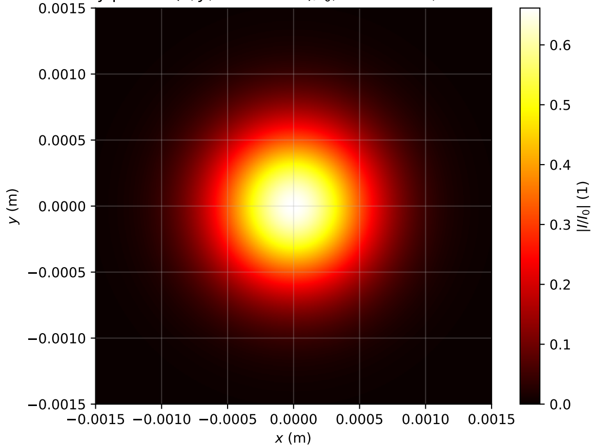
Intensity profile I(x, y, z = 1.751m)/I_0 , Pin=0.2Pcr, artificial time
